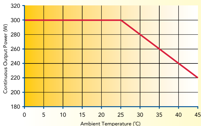
Temperature De-Rate Curve
