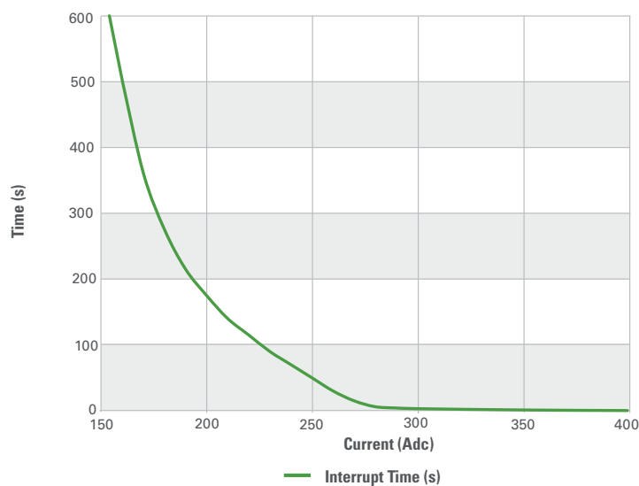
Nominal Interruption Time - Peak Current Characteristic of Discover BMS
