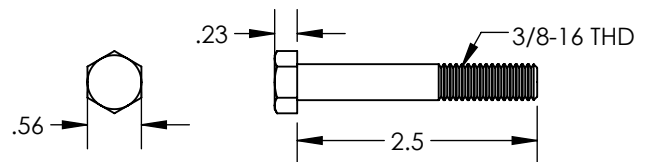
6) Bolt, 3/8-16 X 2.5" CS SS
