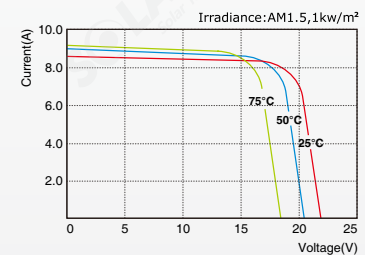
SLP150-12 I-V Curves
